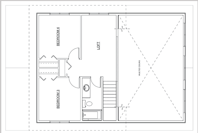
Upper Floor - 541 SQ.FT.
